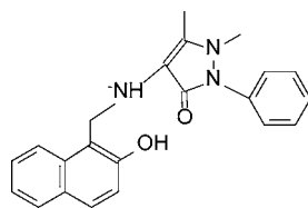
Figure 1. Molecular structure of compound 1 .
