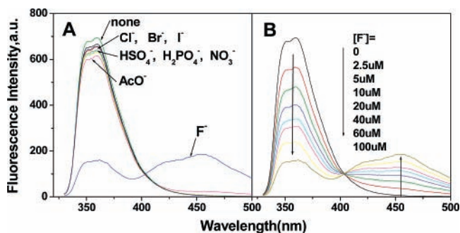
Figure 2. Fluorescence spectra of compound 1 (10 μM) in acetonitrile upon addition of (A) different anions (F – , H 2 PO 4 – , AcO – , HSO 4 – , NO 3 – , Cl – , Br – , I – ) (100 μM) and (B) different concentrations of F – . Excitation wavelength: 320 nm.
