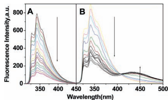
Figure 4. Fluorescence quenching of (A) 1-naphthol (10 \mu M) in acetonitrile upon addition of 4-aminoantipyrine (corrected concentrations: 0, 5, 10, 20, 30, 40, 50, 60, 70, 80, 90, 100, 120, 140, 160, 180, and 200 \mu M) and (B) 1-naphthoxy sodium (10 \mu M) upon addition of different concentrations of 4-aminoantipyrine (corrected concentrations: 0, 5, 10, 20, 30, 40, 50, 60, 70, 80, 90, 100, and 110 \mu M). Excitation wavelength: 300 nm.
