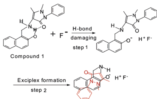
Scheme 1. Schematic Illustration of Breaking of Intramolecular Hydrogen Bonding upon Addition of Fluoride Ion: The Molecular Structure Changes from Rigid to Flexible
