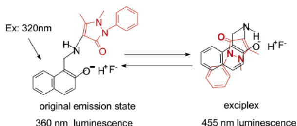
Scheme 2 Fluorescence Decay Process of Compound 1 in Acetonitrile with Two Lifetimes at a Monitored Wavelength of 360 nm
