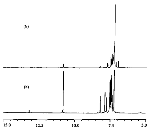
Figure 3. ^1\text{H} NMR (300 MHz) spectra of compound 1 in \text{CD}_3\text{CN} in the presence of 0 (a) and 10 equiv (b) of tetrabutylammonium fluoride.
